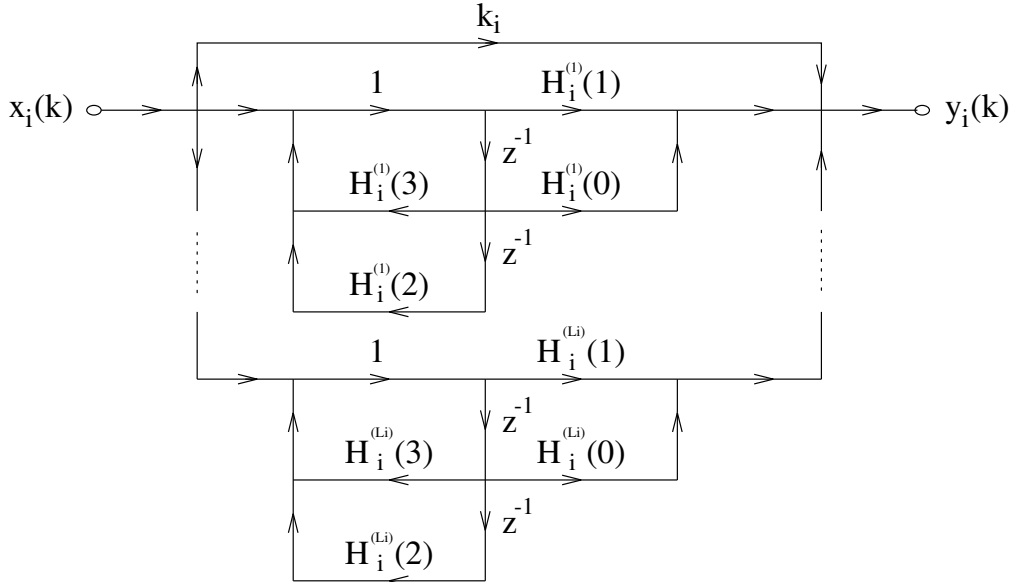
Figure 12.6: MNRU Filters Structure.
