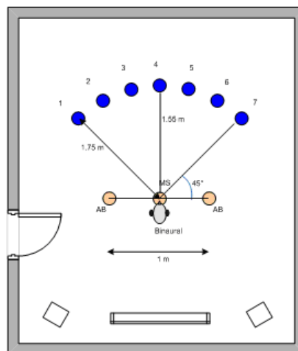
Figure 14.5: Scenario 2 (small video-conference room, AB, MS and Binaural microphones), talker positions 1 through 7, (left though right).
