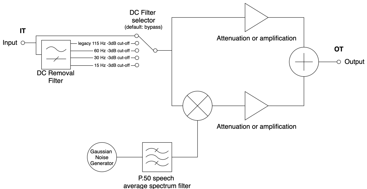
Figure 12.7: P.50 fullband MNRU implementation
