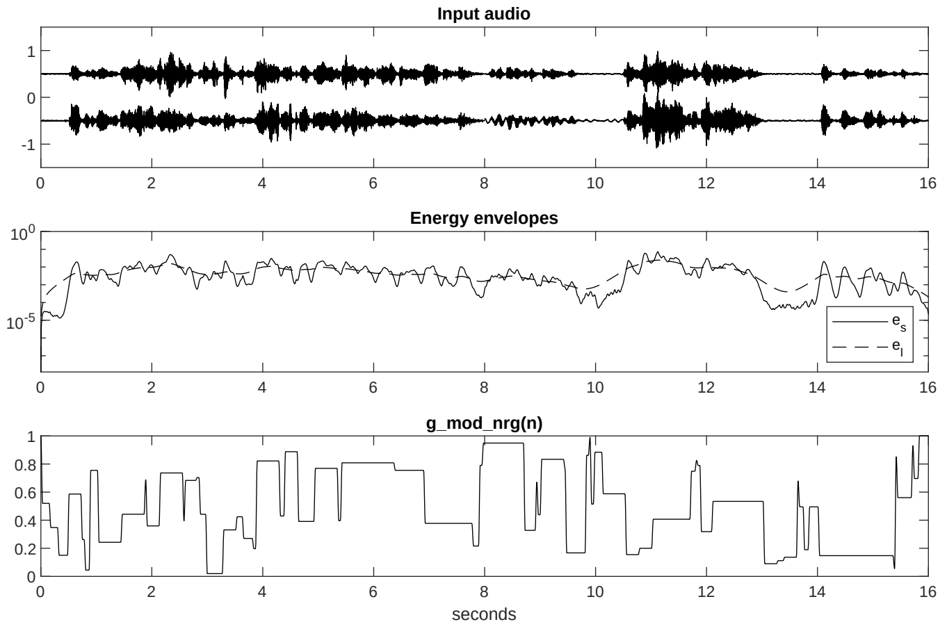
Figure 20.1: The energy of the input file is analyzed and then low-pass filtered to form a short-term estimate e_s(n) and a long-term estimate e_l(n) . When the short-term estimate is above the long-term estimate, e_s(n) > e_l(n) , it is considered a high-energy segment and the change in modulation is limited by e_{step} .
