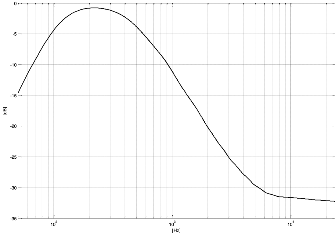
Figure 12.8: Frequency response of noise shaping filter.
