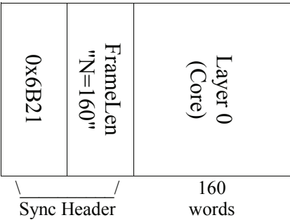
Figure 11.8: Example G.192 output frame when layer 1, layer 3 and layer 4 are hit by layer errors in the layered error application mode.
